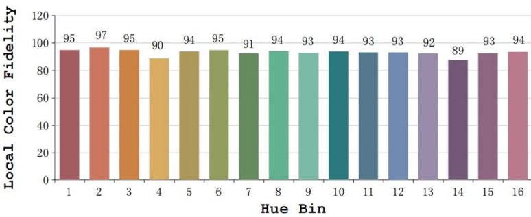
TM-30 2700K
